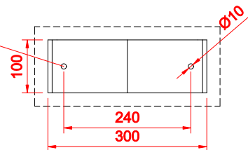
MOUNTING HOLES SPACING
